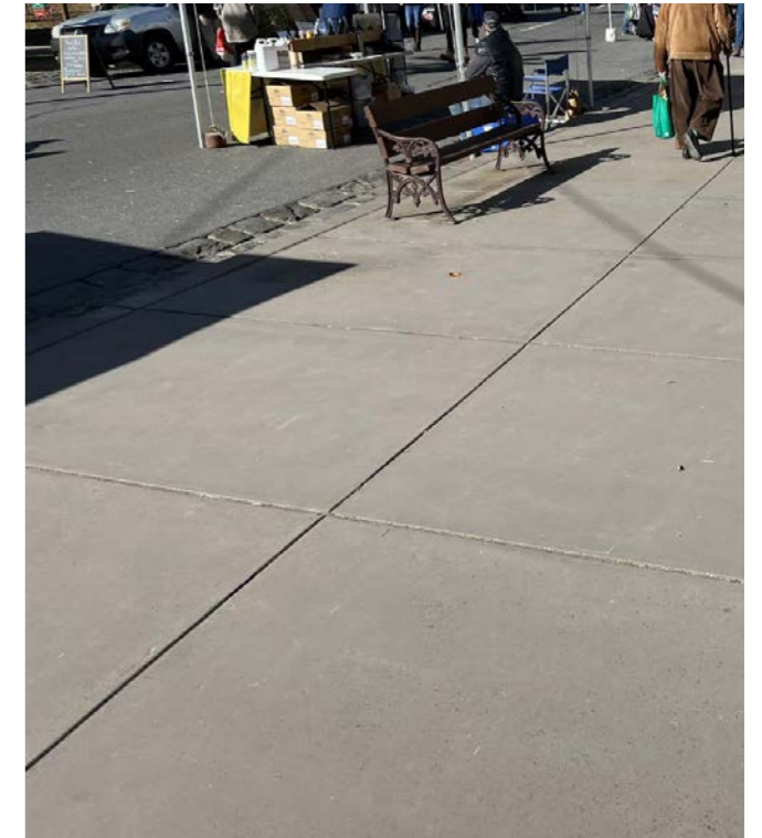
Typical Concrete Pavement with tool joints
